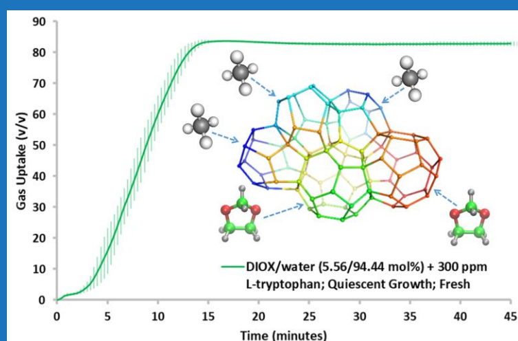
Ultra-rapid mixed methane-DIOX (sII) hydrate formation
