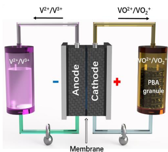
Left: Configuration of CARB battery with PBA loaded in the catholyte tank; Middle: Operation temperature, electrolyte \text{VO}_2^+ and acid concentration of VRB and CARB batteries; Right: Roadmap of various redox-targeting-based RFBs and comparison with other battery technologies.
